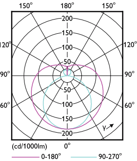
Light Distribution Diagram - 14.5T8/COR/48-830/MF20/G 10/1
