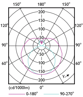
Light Distribution Diagram - 44T8HO/COR/96-840/MF54/G/R17d 10/1
