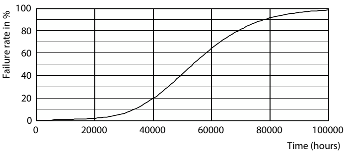
Life Expectancy Diagram - 11T5HE/34-830/IF14/G/DIM 10/1
