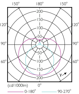
Light Distribution Diagram - 11T5HE/34-830/IF14/G/DIM 10/1
