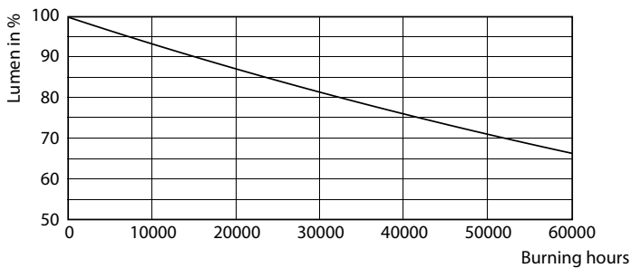
Lumen Maintenance Diagram - 11T5HE/34-830/IF14/G/DIM 10/1
